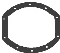
Part # EQ-006, 1/16 N/C Part # EQ-006-1, 1/16 Neo R750/R1600 Hand Hole Gasket
