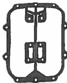
Part # EQ-019 Ref.# 001-62-163-23 # 1 Valve Plate 1/16 Neo/Cork
