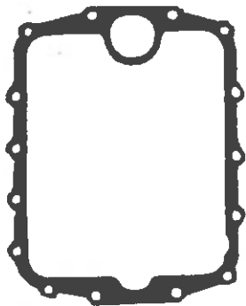
Part # AM-044 Ref.# 44094P002 AL800/1000, 100LB Top 1/16 Neoprene
