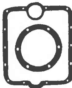
Part # AM-103C Includes AM-004 & AM-030 AL800/1000 Hand Hole & Top Gasket 1/16 Neoprene
