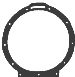
Part # SP-007, 1/16 N/C Part # SP-007-1, 3/64 N/C Ref.# 015270 1A/175 Iron, Side Plate
