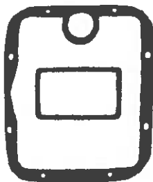
Part # AM-101C Includes AM-009 & AM-018 Index Box & Top Gasket 1/16 Neo/Cork
