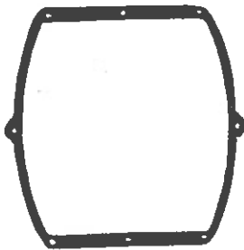
Part # AM-038 Ref.# 39663P001 5B 225, 8 Hole 1/16 Neo/Cork
