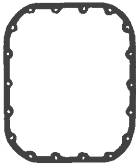
Part # EQ-034, 1/16 N/C Part # EQ-034-1, 1/16 Neo Ref.# 011-14-164-12 R750 Top Cover
