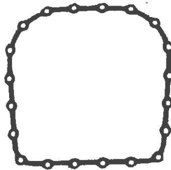
Part # AM-045 Ref.# 44639P001 AL800/1000, 100LB Side 1/16 Neoprene
