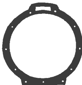
Part # SP-008, 1/16 N/C Part # SP-008-1, 3/64 N/C Ref.# 065270 175, 240 & 250 Iron/Alum
