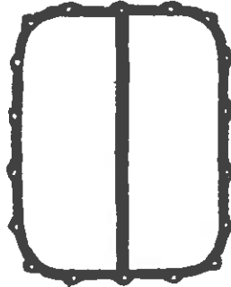
Part # EQ-032 Ref.# -11-14-163-00 R750/R1600 Valve Plate 1/16 Neo/ Cork
