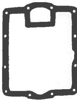
Part # AM-027 1/16 Neo/Cork Part # AM-028 1/16 Neoprene Ref.# 44275P001 AL 425
